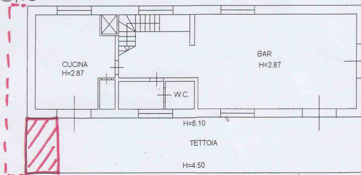
PIANO TERRA
