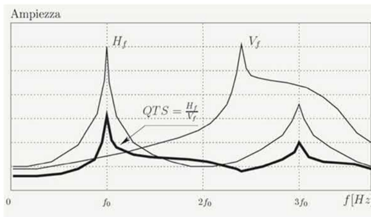
Horizontal-to-Vertical Spectral Ratio from passive seismic
